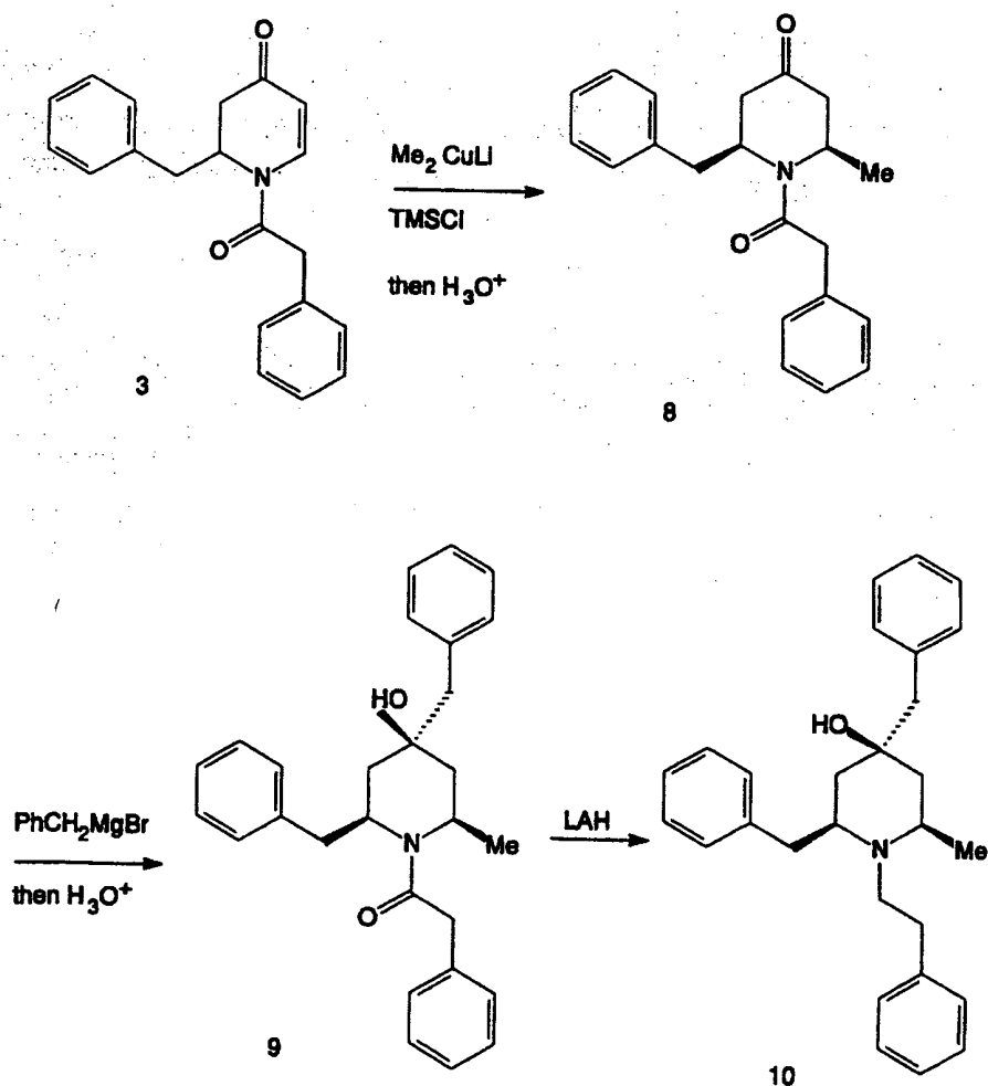
Scheme 4
